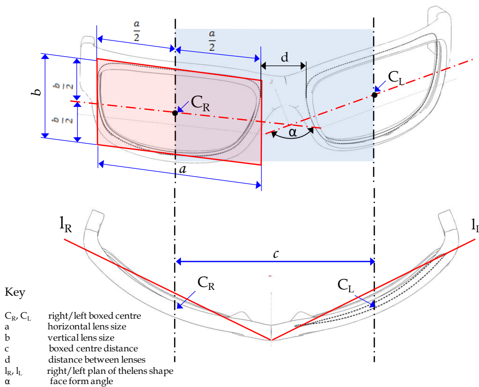
Figure 1b) Measurements of the boxed lens size, made in the plane of the lens shape and measurements of distance between lenses , made in the plane of spectacle front
