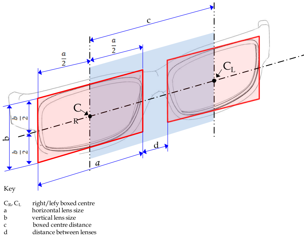
Figure 1 Measurements of the boxed lens size and distance between lenses , made in the plane of spectacle front
